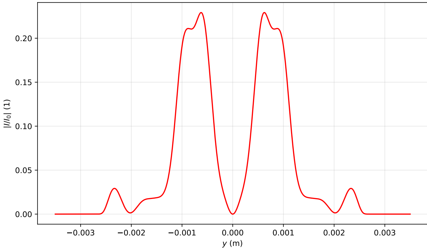
Intensity profile I(x=0, y, z=3.742)/I_0 , P_{in}=6.0P_{cr} , artificial time
